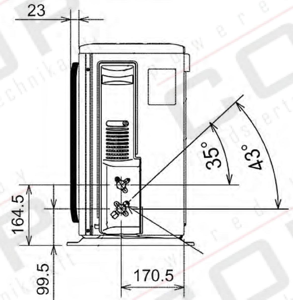
Side View >
